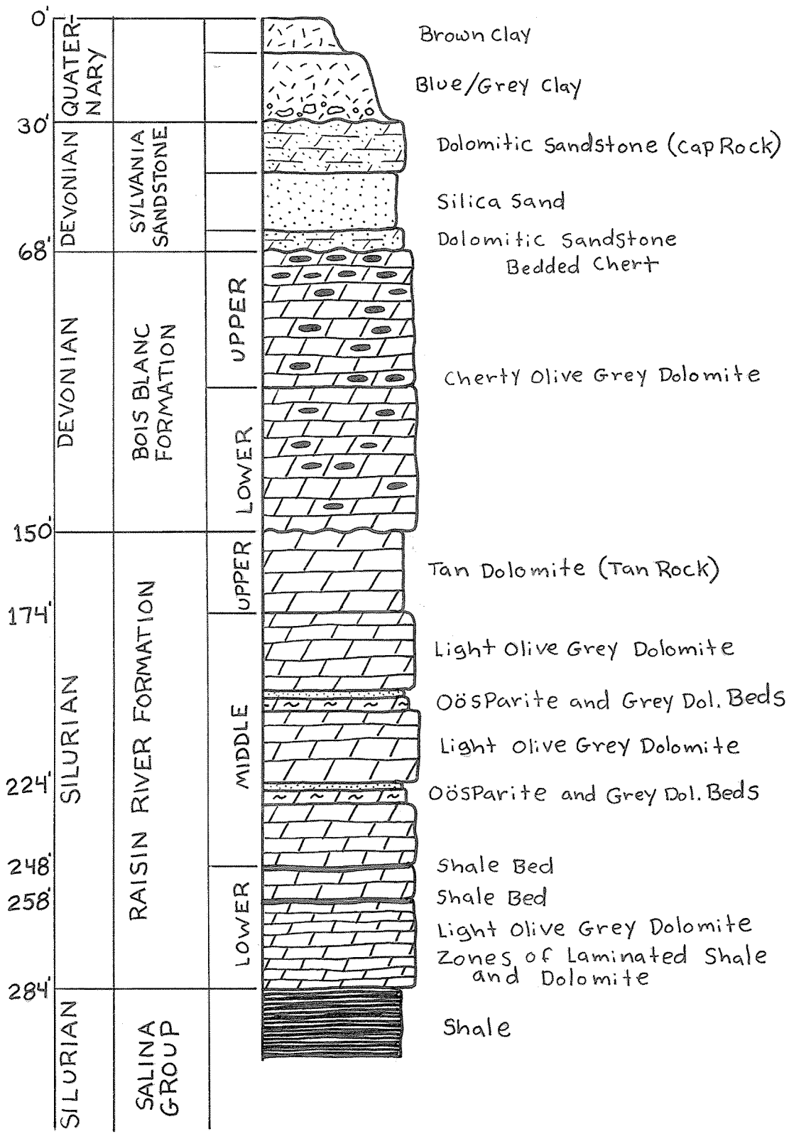
Figure 2.1 Sylvania Minerals Stratigraphic Succession, Typical Scale: 1 inch = 40 feet
